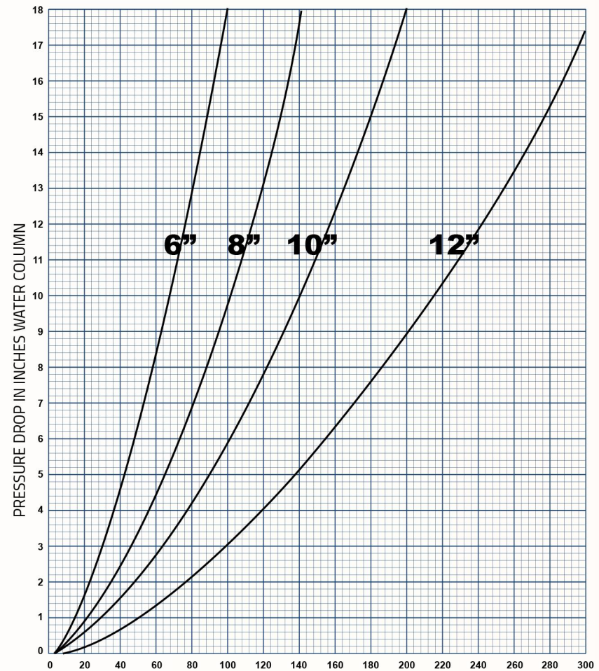
AIR FLOW IN STANDARD CUBIC FEET PER HOUR X 1,000 FLOW CAPACITY CURVE FOR FAV SYSTEMS INC. DETONATION FLAME ARRESTORS MODELS 6", 8", 10" & 12" ILSF-A DA, ILSF-B DA OR ILNF-DA
