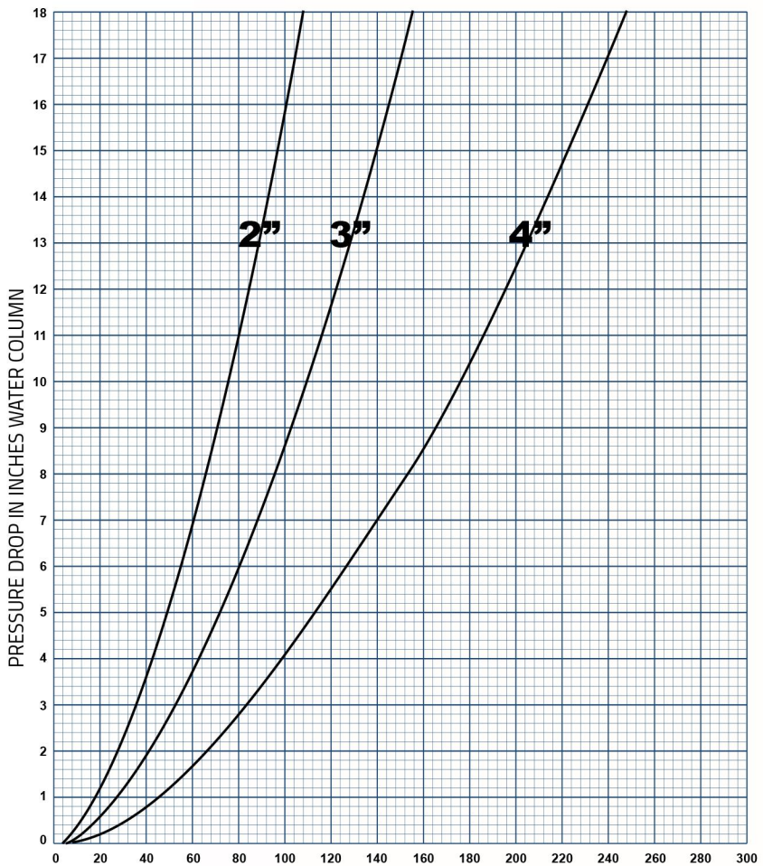
AIR FLOW IN STANDARD CUBIC FEET PER HOUR X 1,000 FLOW CAPACITY CURVE FOR FAV SYSTEMS INC. DETONATION FLAME ARRESTORS MODELS 2", 3" & 4" ILSF-A DA, ILSF-B DA OR ILNF-DA
