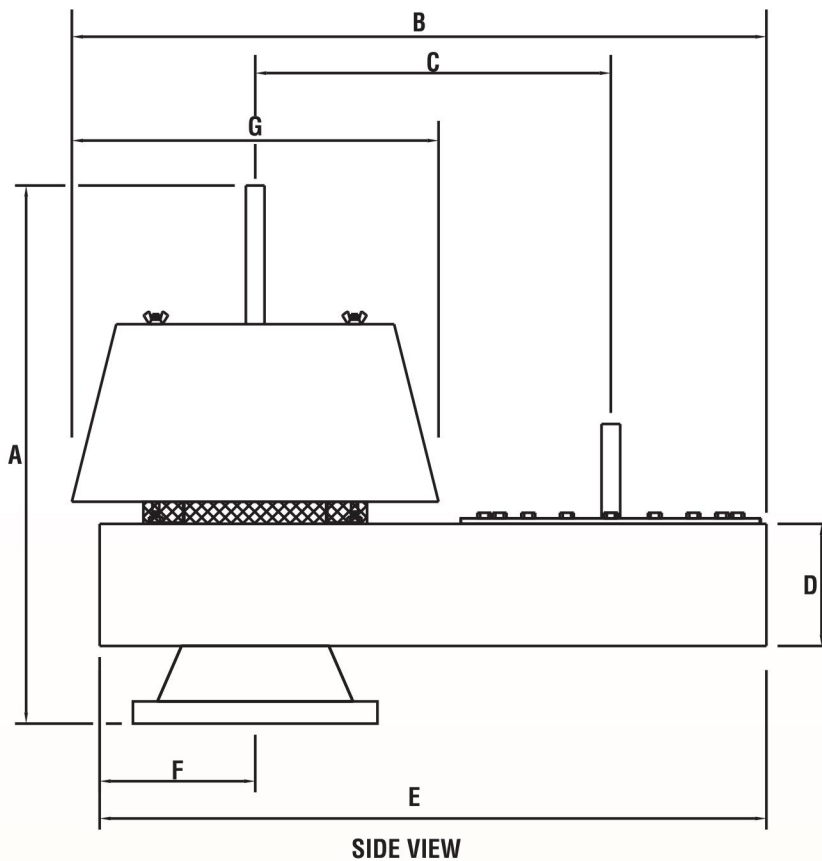
FAV SYSTEMS MODEL P.V.T.A. (Pressure Vacuum To Atmosphere)
