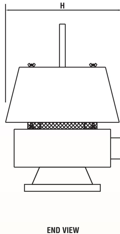
FAV SYSTEMS MODEL P.V.T.A. (Pressure Vacuum To Atmosphere)
