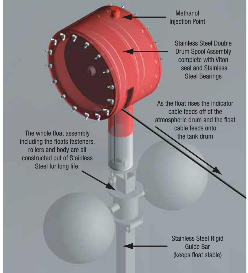
Float Assembly
