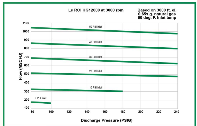
Compressor Curves Available
